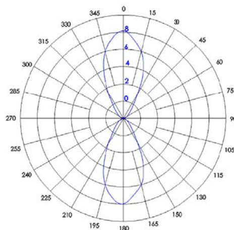
E-plane Co-polarization Pattern
